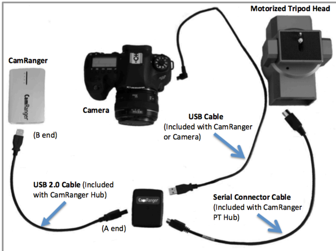
Diagram of setup for the CamRanger, CamRanger PT Hub, motorized tripod, and camera.
